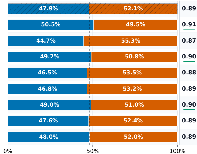
Qwen2.5-7B
