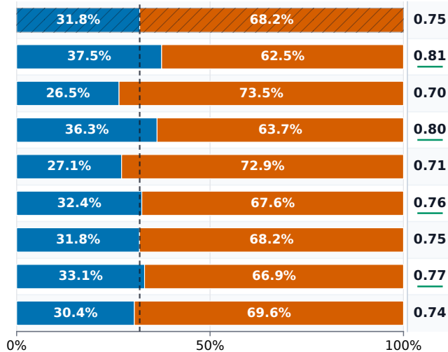
Qwen2.5-3B
